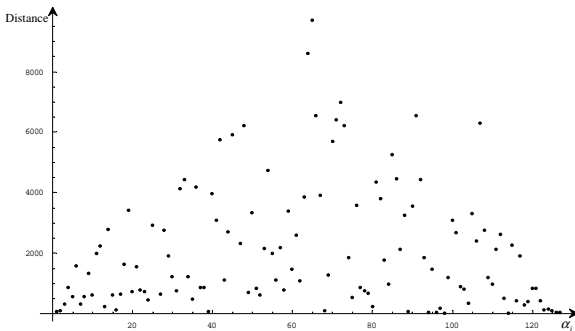
Figure 1: Differences between \|a + \alpha\| and \|a\|
